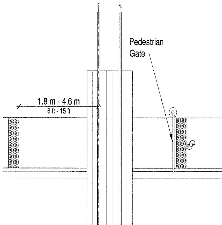
Figure R305.2.5 Pedestrian At-Grade Rail Crossings
