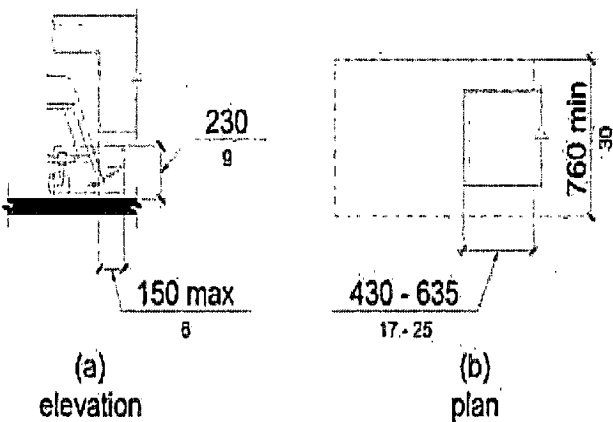
Figure R405.2 Toe Clearance
