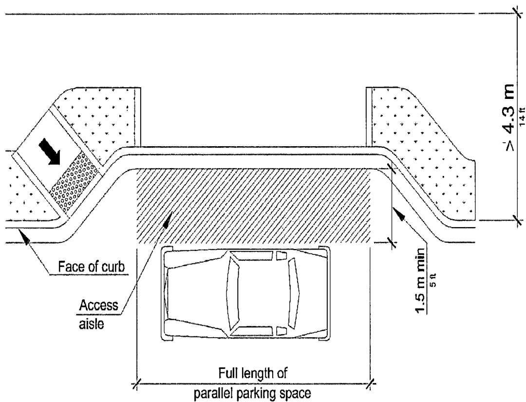
Figure R309.2.1 Wide Sidewalks
