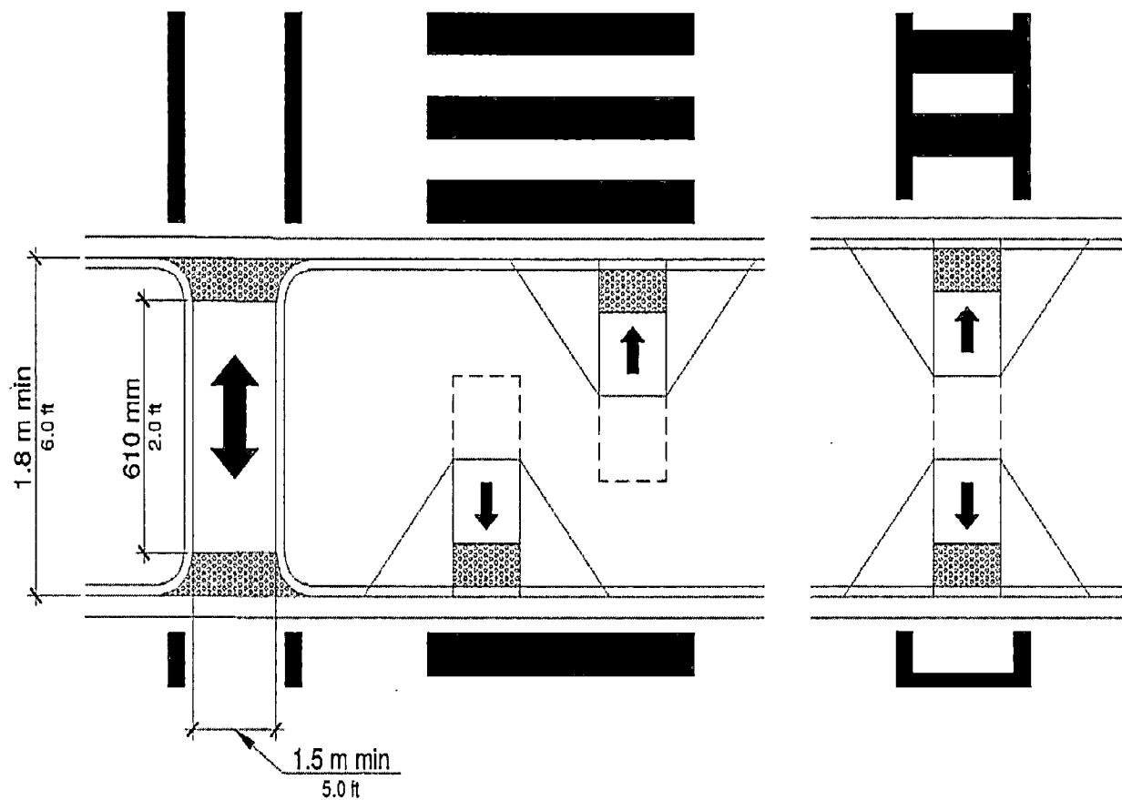
Figure R305.2.4 Pedestrian Refuge Islands
