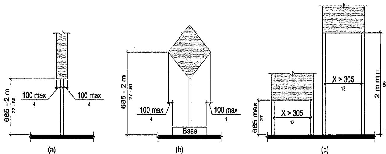
Figure R402.3 Post-Mounted Objects
