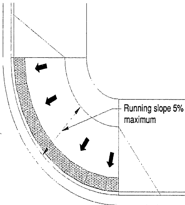
Figure R304.4.1 Running Slope
