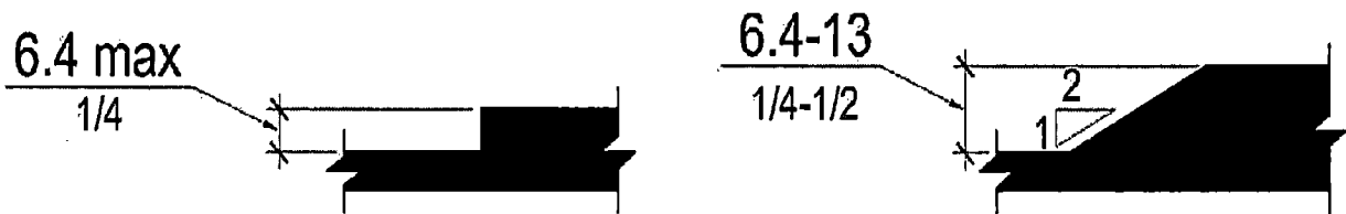
Figure R302.7.2 Vertical Surface Discontinuities
