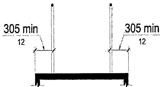
Figure R407.9.1 Extended Ramp Surface
