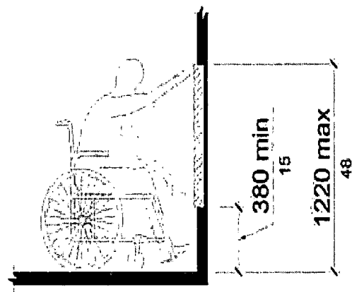
Figure R406.2 Unobstructed Forward Reach
