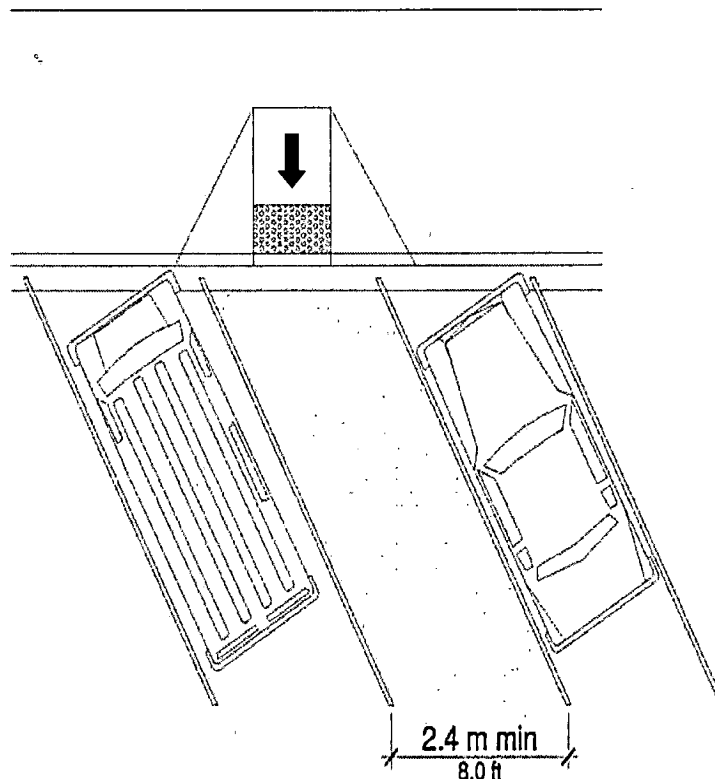
Figure R309.3 Perpendicular or Angled Parking Spaces
