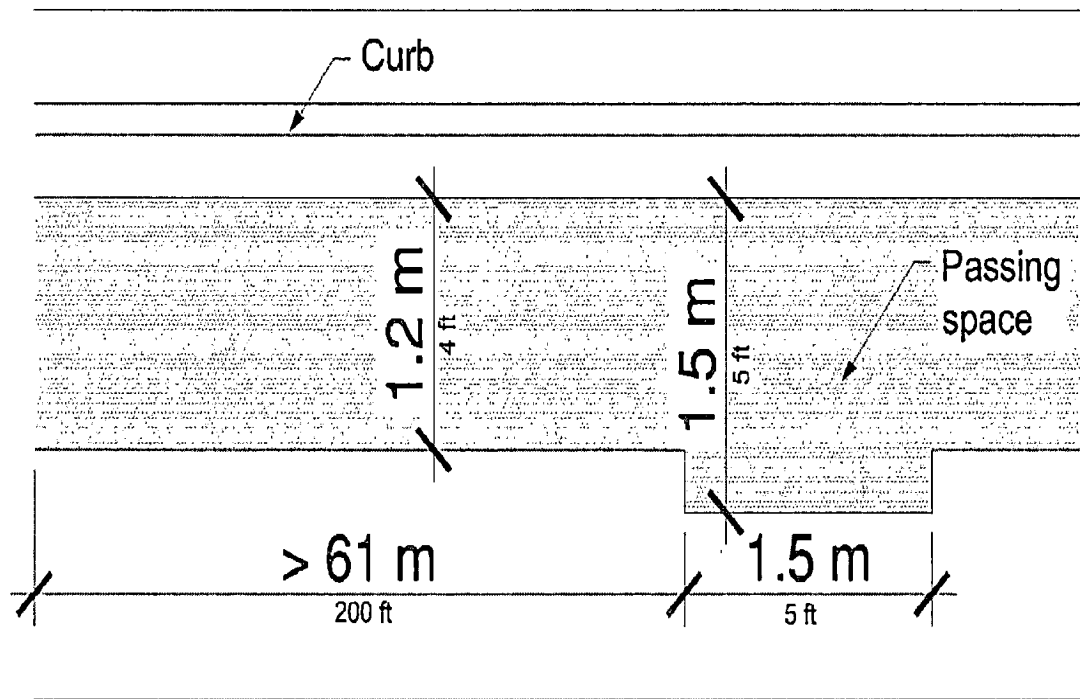
Figure R302.4 Passing Spaces
