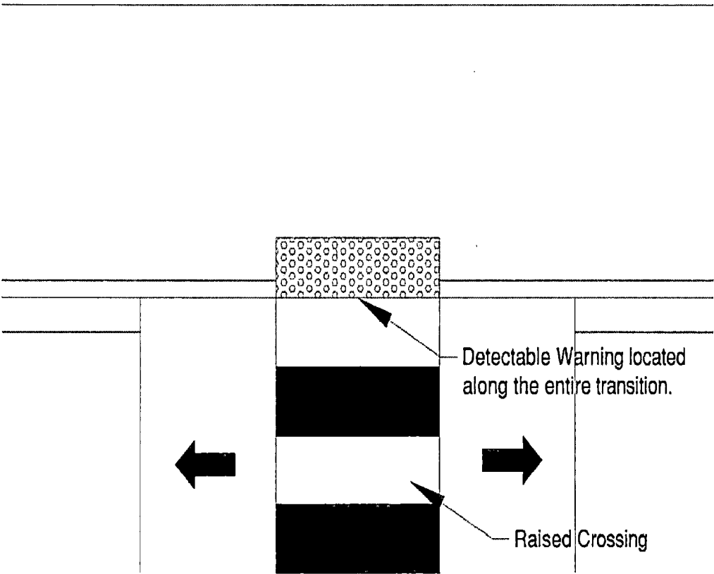
Figure R305.2.3 Blended Transitions
