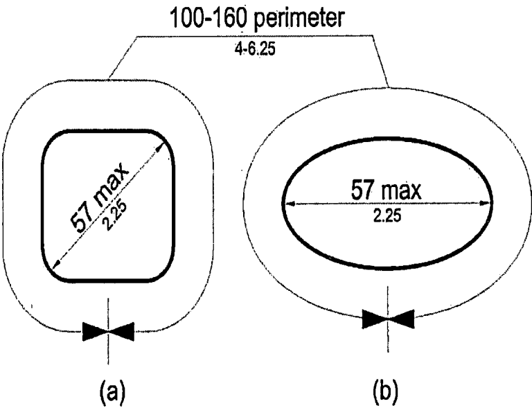
Figure R409.7.2 Non-Circular Cross Sections
