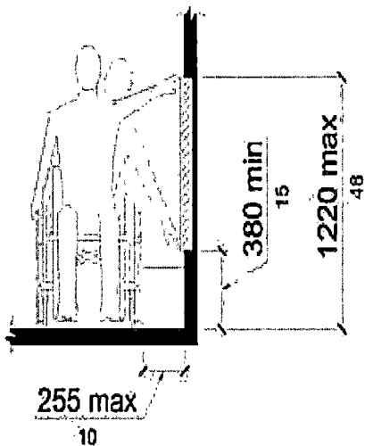
Figure R406.3 Unobstructed Side Reach
