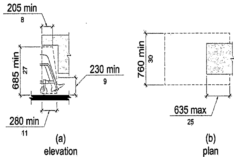
Figure R405.3 Knee Clearance
