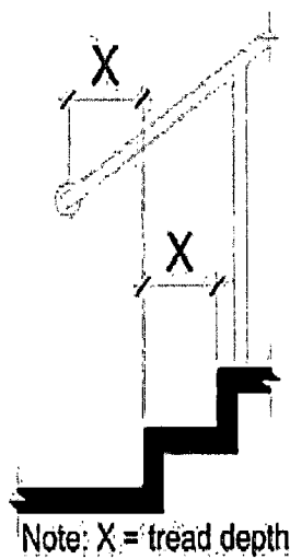
Figure R409.10.3 Bottom Extension at Stairways
