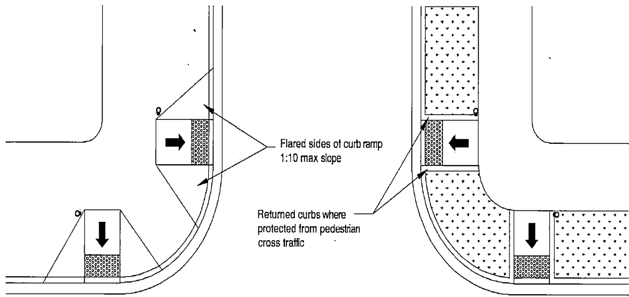
Figure R304.2.3 Flared Sides
