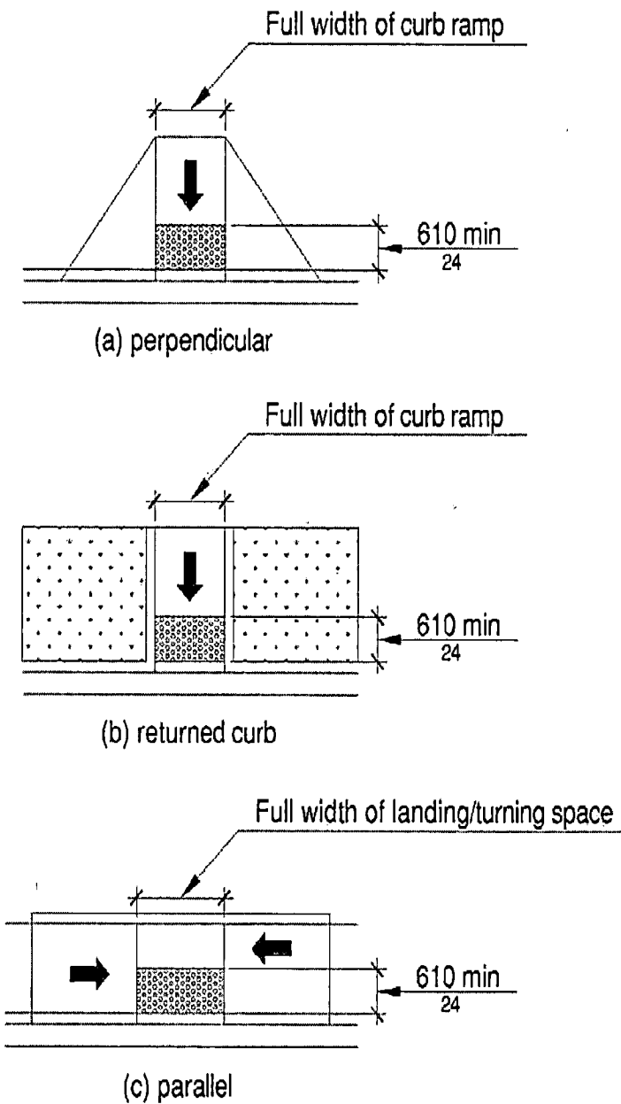
Figure R305.1.4 Size
