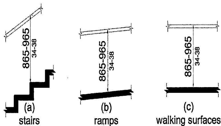
Figure R409.4 Height
