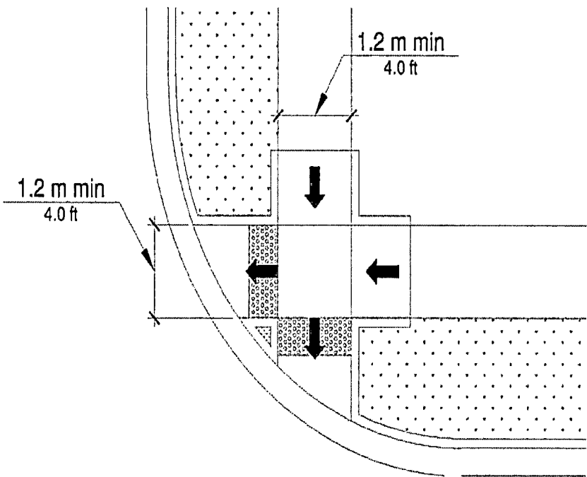
Figure R304.5.1 Width
