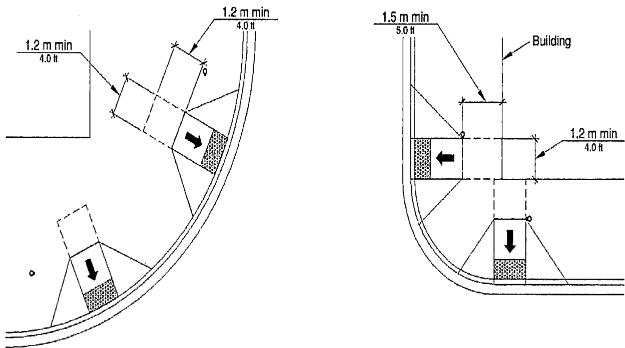
Figure R304.2.1 Turning Space
