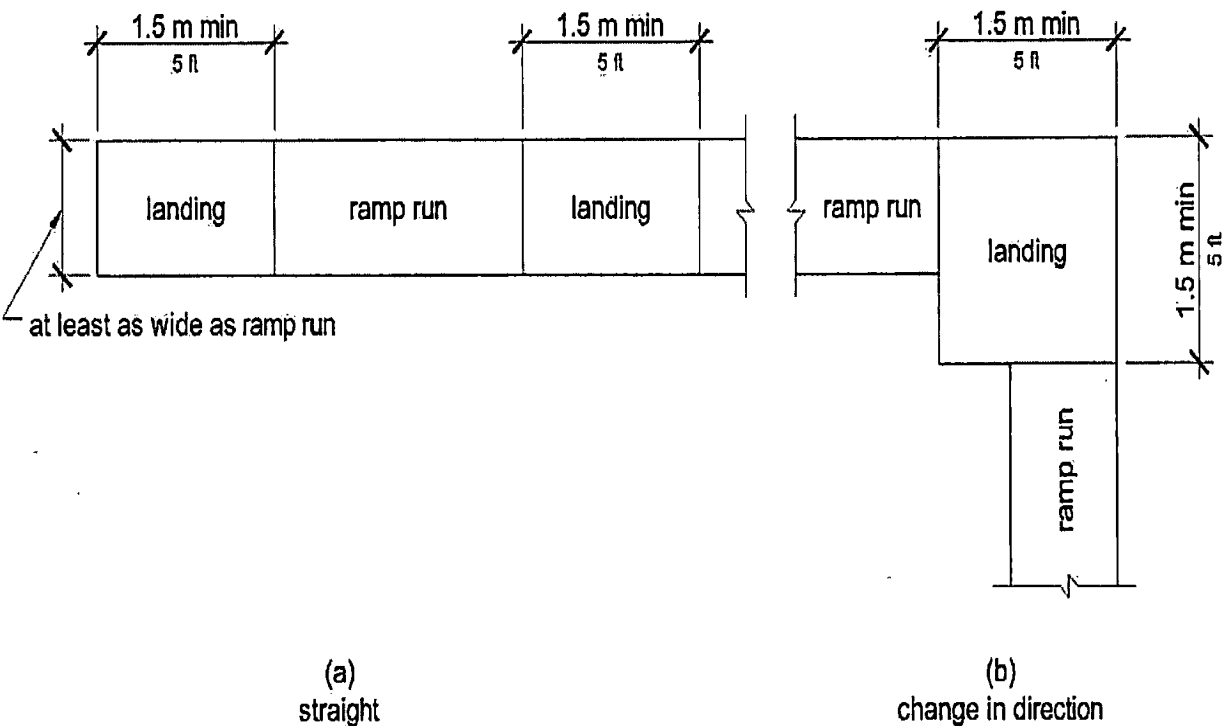
Figure R407.6 Landings
