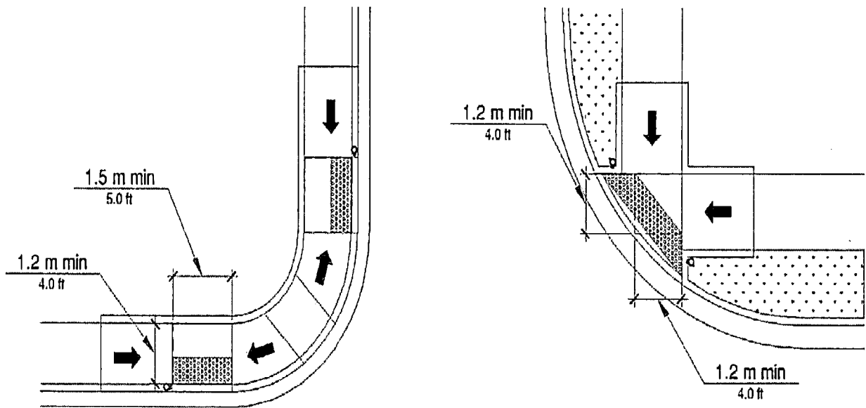
Figure R304.3.1 Turning Space
