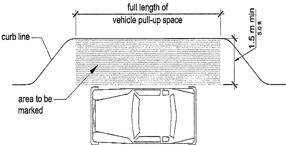
Figure R310.3 Access Aisle
