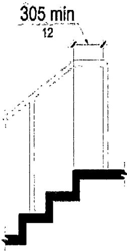
Figure R409.10.2 Top Extension at Stairways
