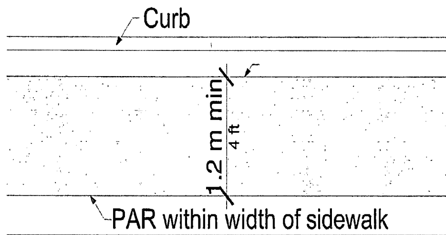
Figure R302.3 Continuous Width
