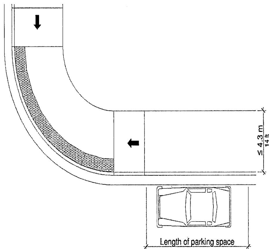
Figure R309.2.2 Narrow Sidewalks
