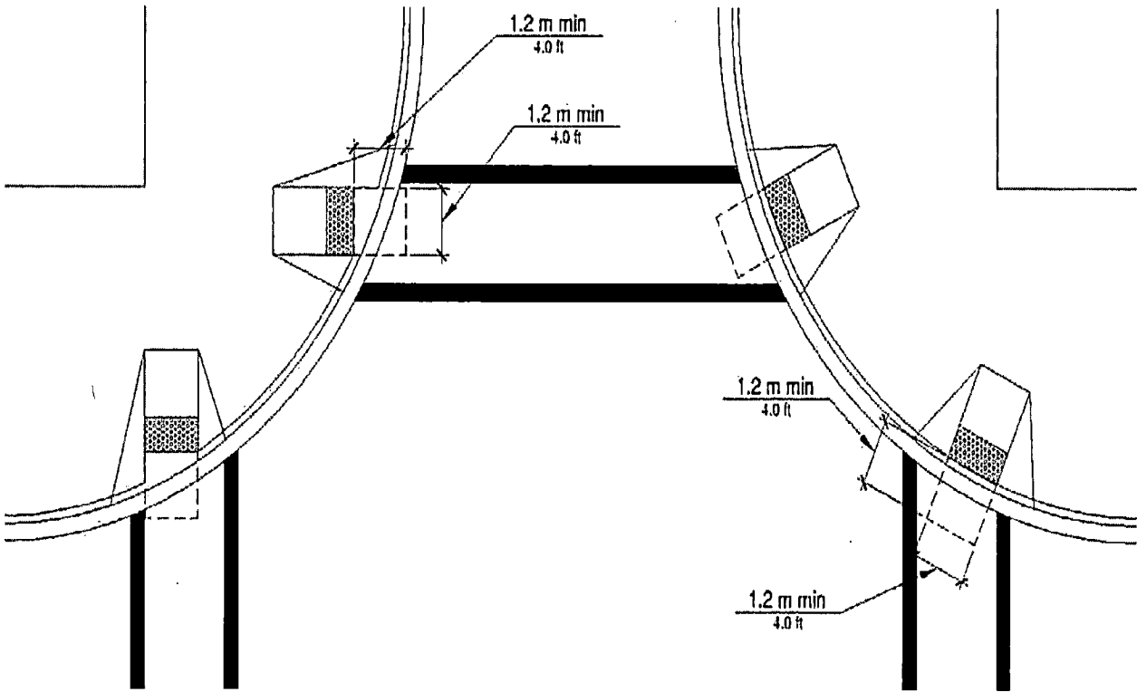
Figure R304.5.5 Clear Space
