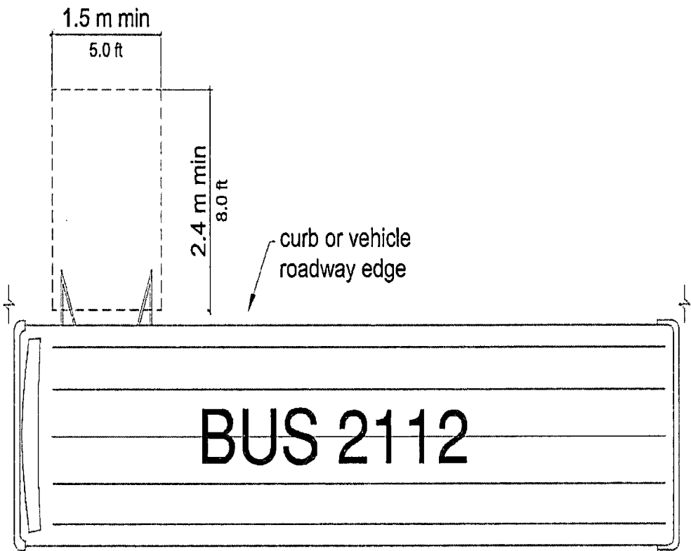
Figure R308.1.1.1 Dimensions
