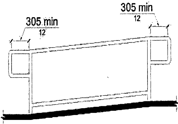
Figure R409.10.1 Top and Bottom Extension at Ramps
