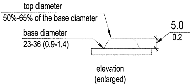
Figure R305.1.1 Dome Size
