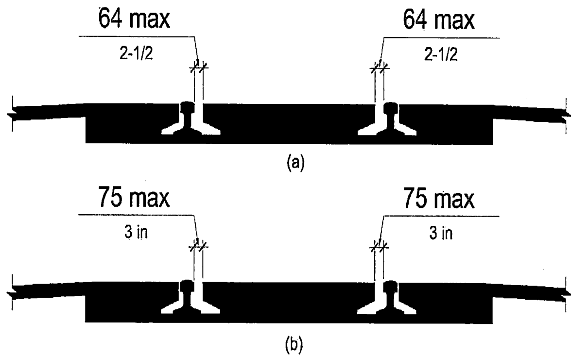
Figure R302.7.4 Flangeway Gaps
