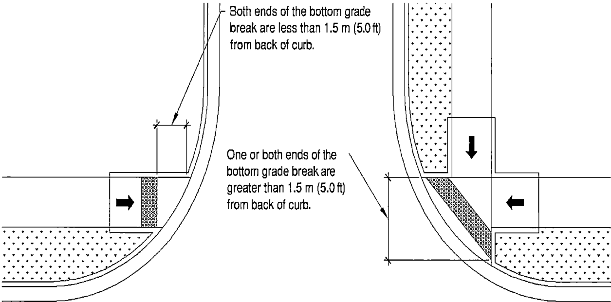
Figure R305.2.1 Perpendicular Curb Ramps
