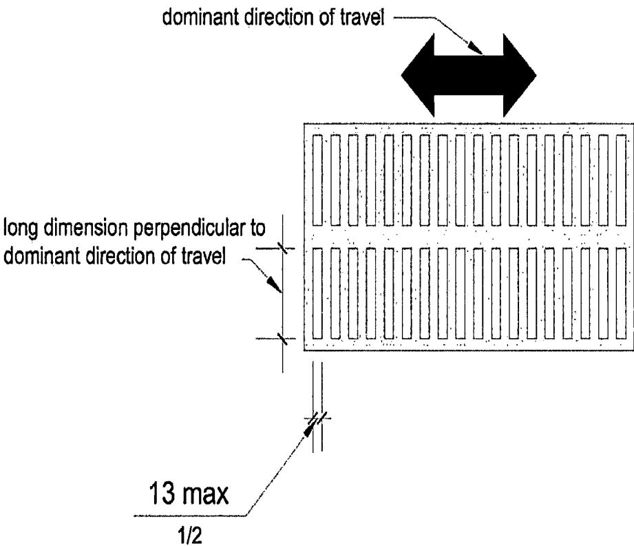
Figure R302.7.3 Horizontal Openings
