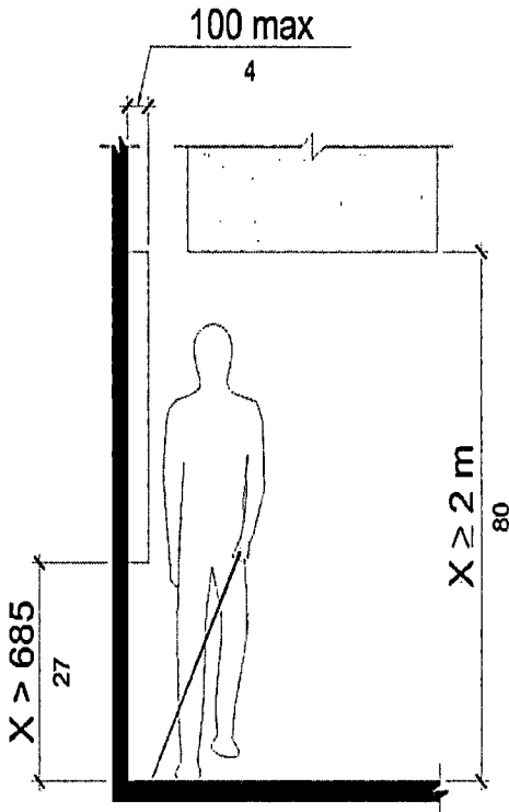
Figure R402.2 Protrusion Limits
