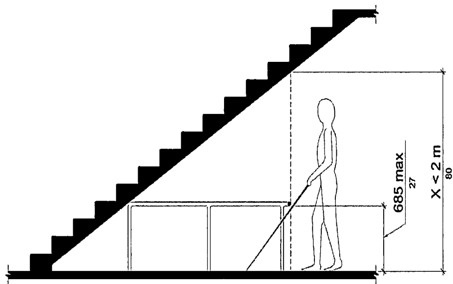
Figure R402.4 Reduced Vertical Clearance
