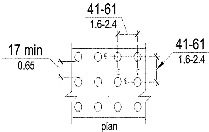
Figure R305.1.2 Dome Spacing
